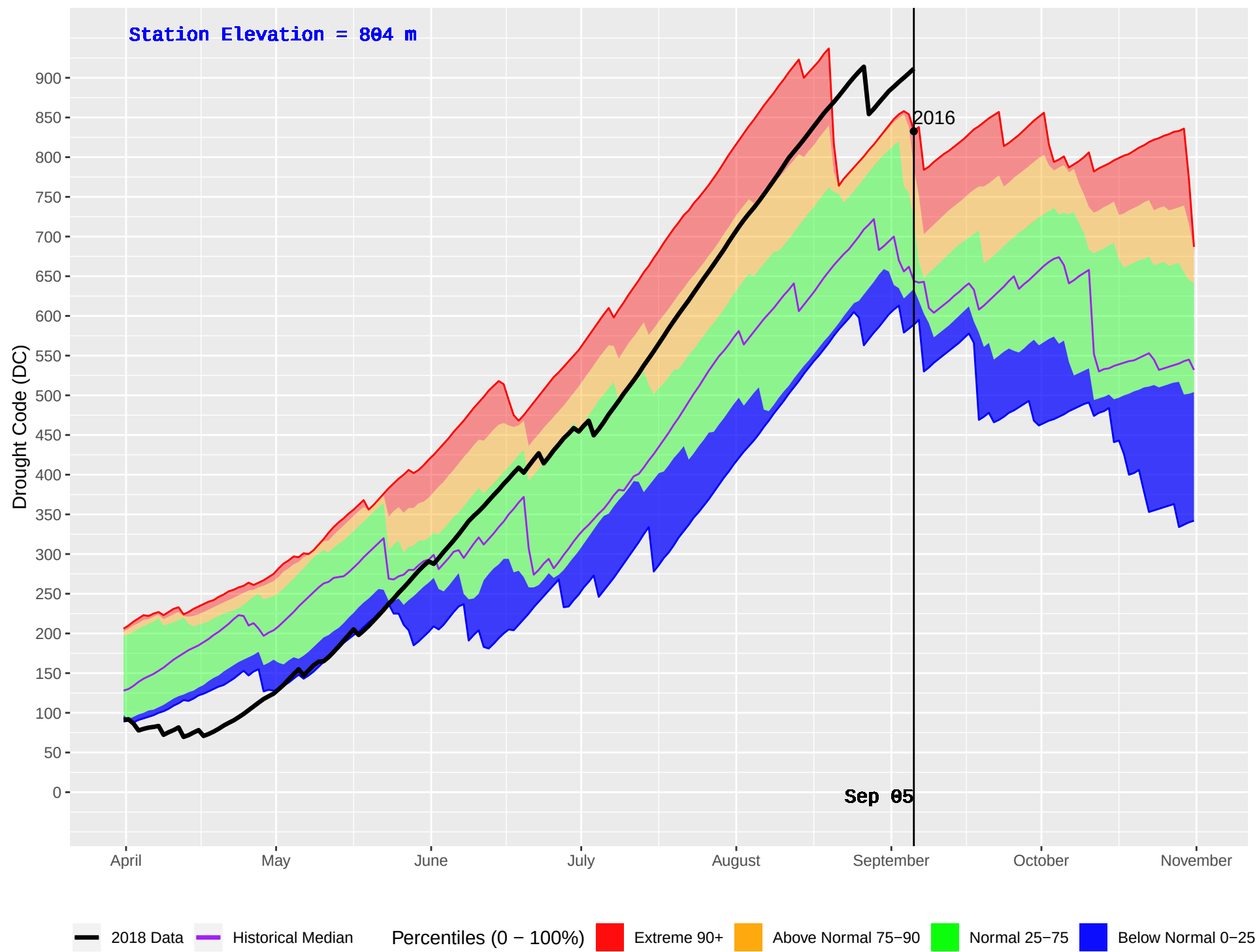
KOOCANUSA (1075) : Historical (2010–2016) and Current (2018) Daily Drought Code (DC)
